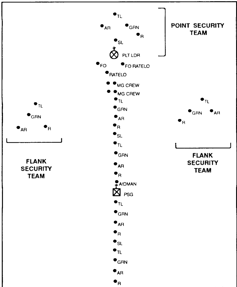
Figure 2-16. Platoon file.
